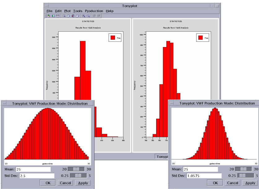
Yield analysis with user selectable statistical distribution. Yield of ring oscillator frequency is shown as a function of different process parameter distribution.
