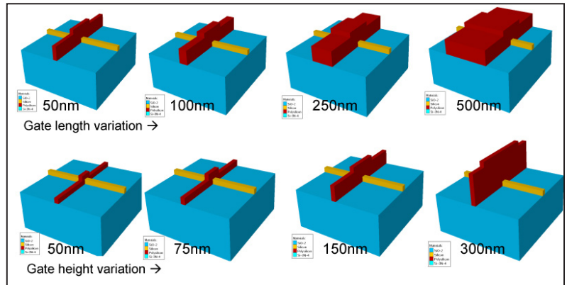
3D FinFET results from many runs showing gate length and height variations. Silicon nitride capping layer is not shown.
