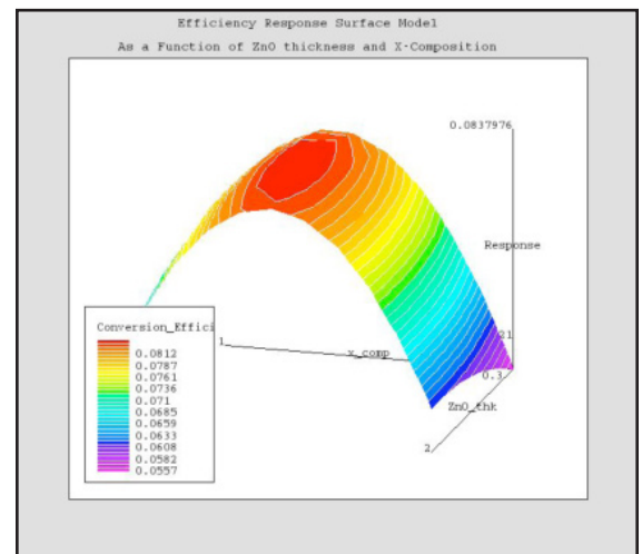
This example shows the Solar Cell Efficiency "Response Surface" using the two variables ZnO thickness and X-Composition. This makes it simple to read off optimum values for cell efficiency.
